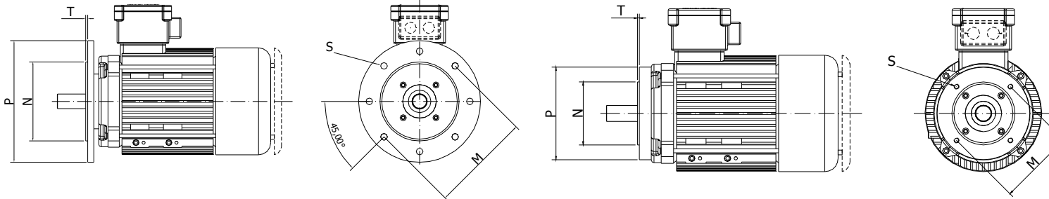
Mounting B5
