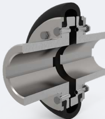
Shaft Coupling with longer hub
